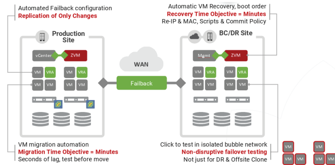
Backup Scenarios with Backup Server
